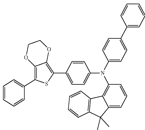
Compound 29
