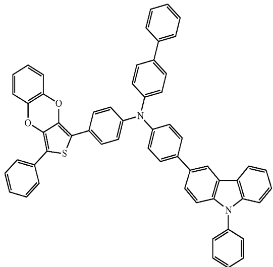
Compound 102
