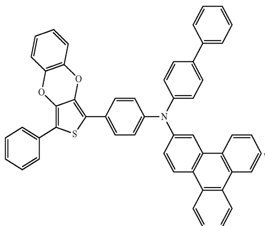
Compound 104
