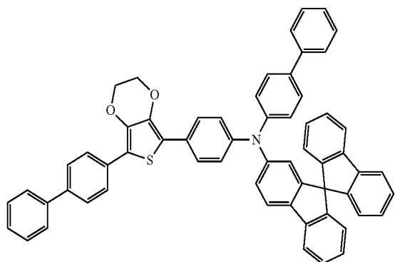
Compound 41
