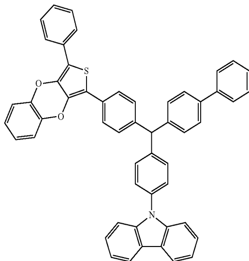
Compound 103
