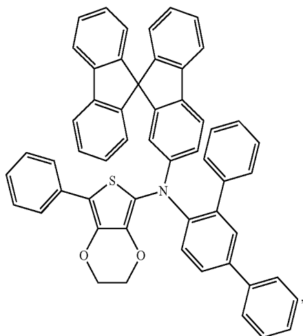
Compound 9
