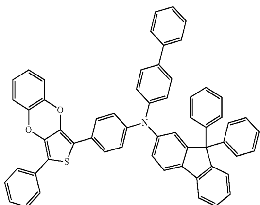
Compound 85
