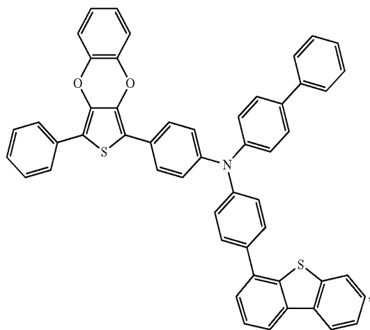
Compound 100
