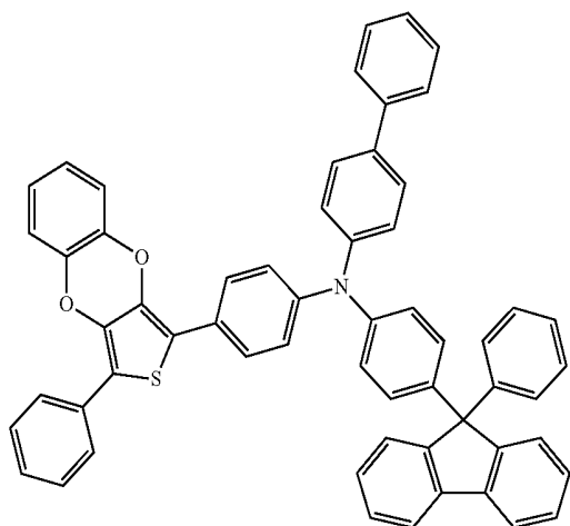
Compound 91
