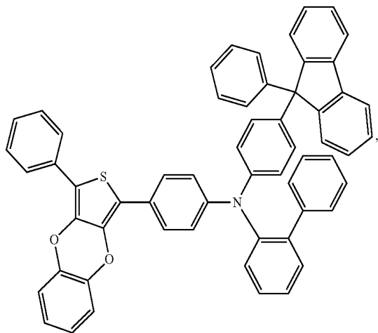
Compound 92
