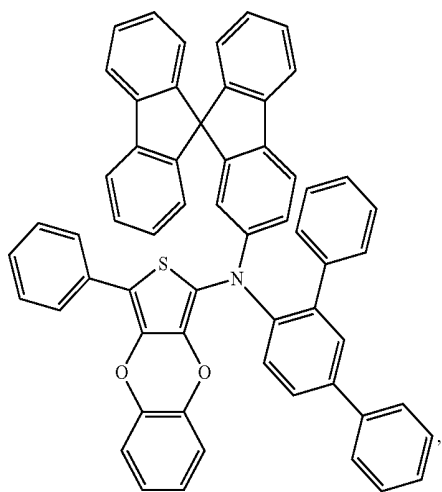
Compound 64
