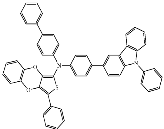
Compound 74
