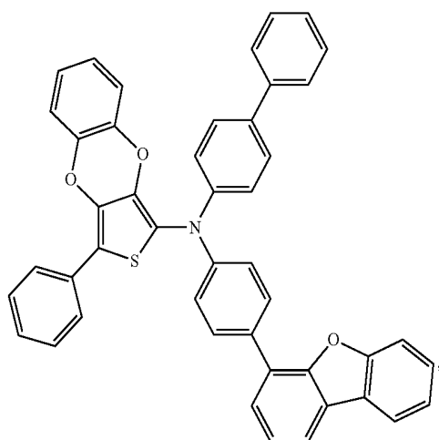
Compound 70
