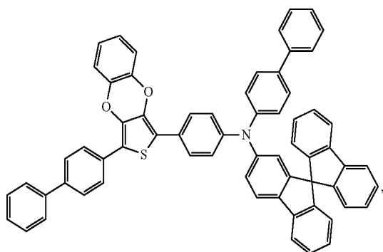
Compound 94
