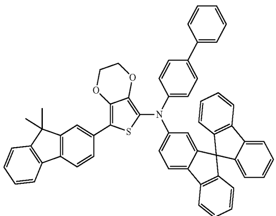
Compound 14
