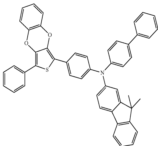
Compound X
