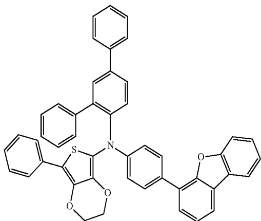
Compound 16
