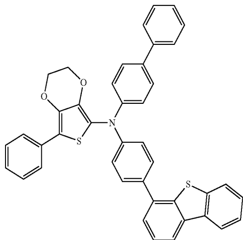
Compound 18
