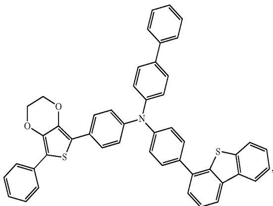
Compound 46
