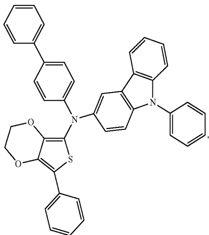
Compound 21
