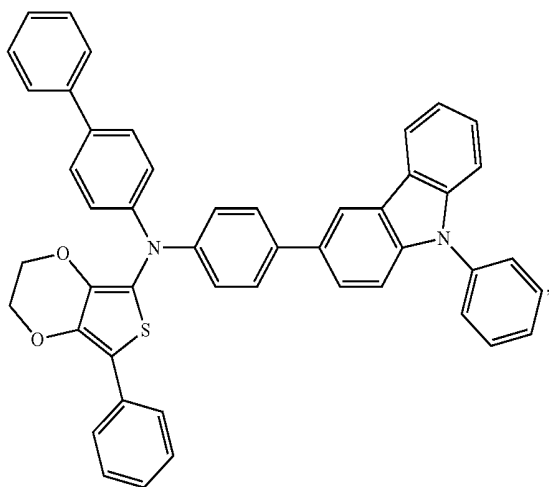
Compound 21
