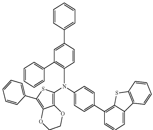
Compound 19
