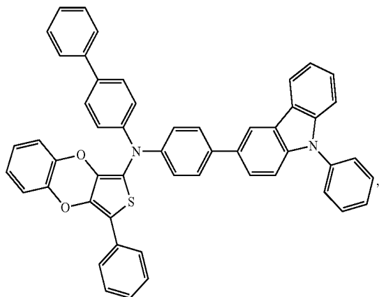
Compound 74
