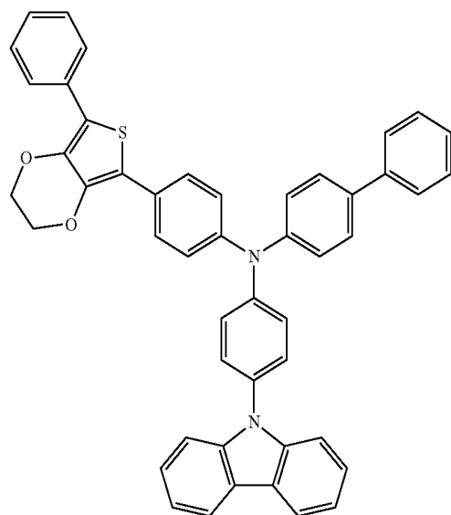
Compound 49
