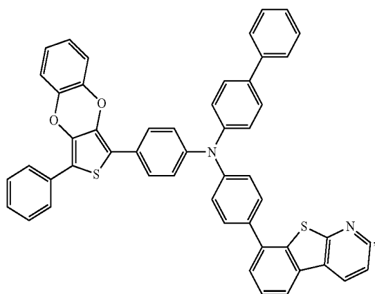
Compound 105
