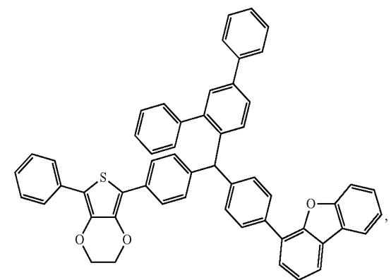
Compound 43
