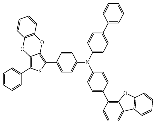
Compound 96
