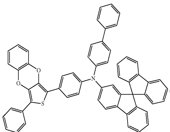
Compound 88
