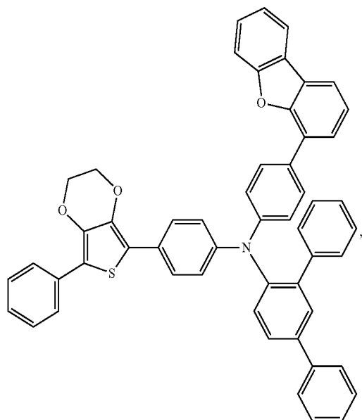
Compound 46
