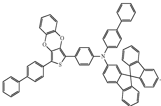
Compound 94
