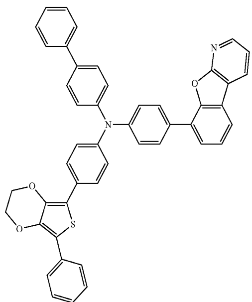
Compound 52
