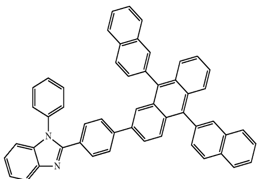
Compound ET
