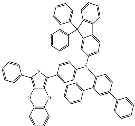
Compound 88
