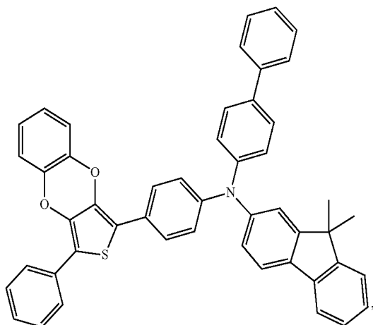
Compound 82
