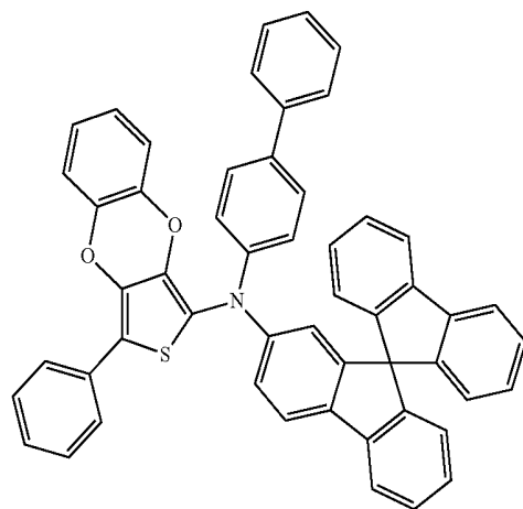
Compound 61
