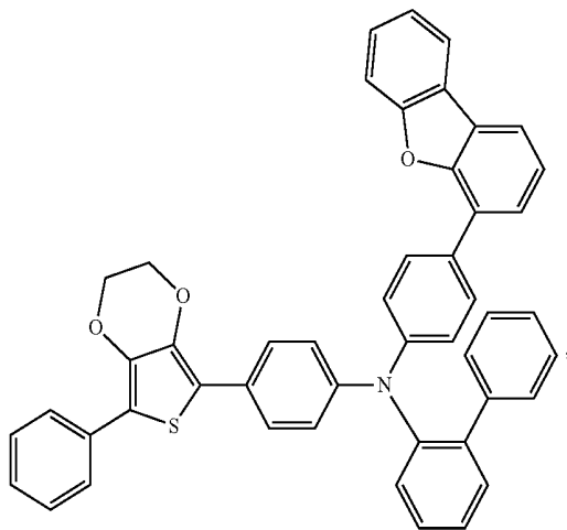
Compound 44
