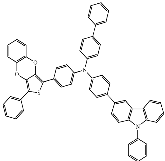
Compound 102
