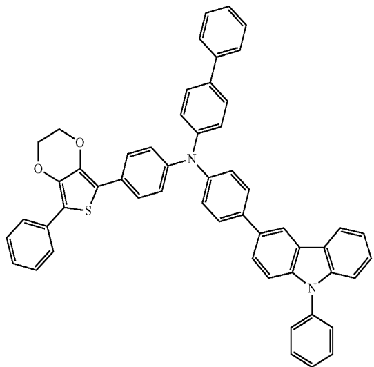
Compound 48
