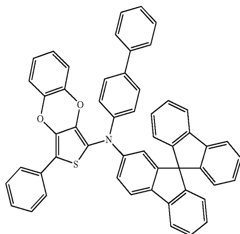
Compound 61
