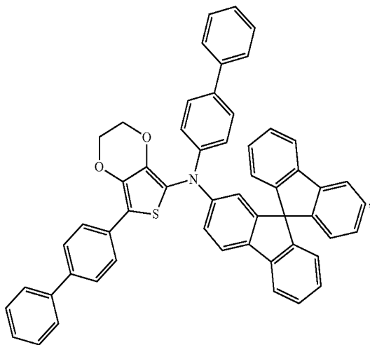
Compound 13
