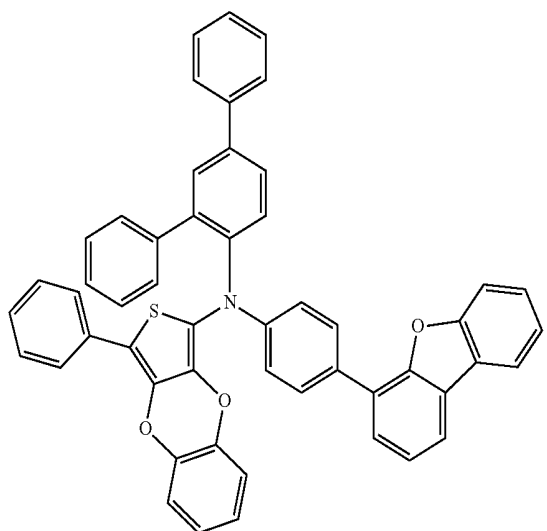
Compound 70
