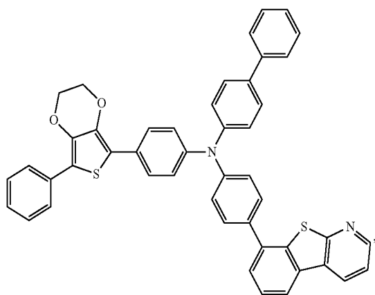
Compound 52
