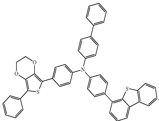
Compound 46
