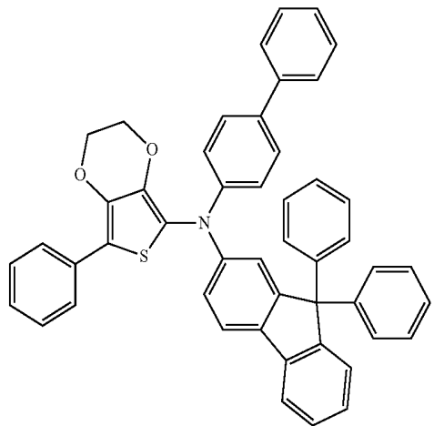
Compound 4
