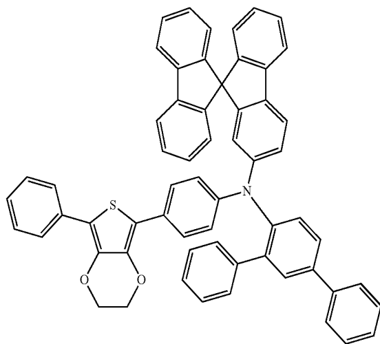
Compound 36
