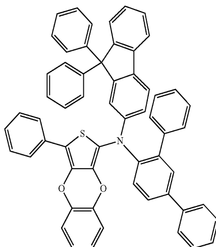
Compound 60
