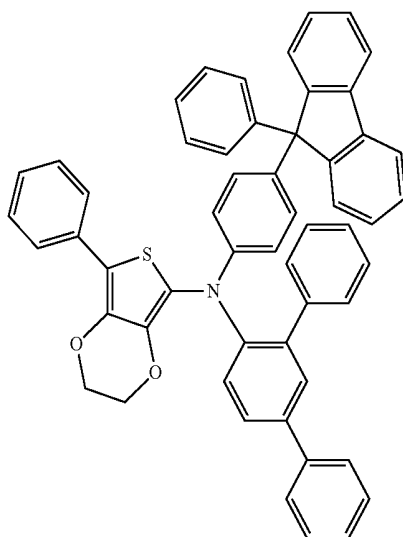
Compound 9
