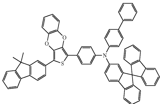
Compound 95
