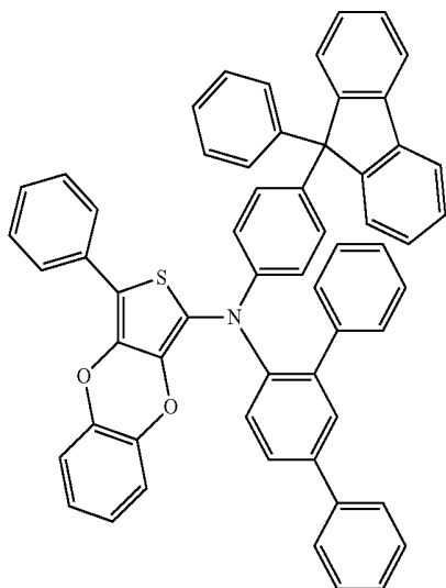
Compound 63
