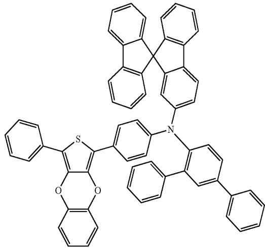
Compound 91
