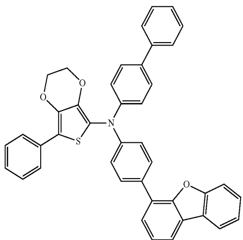
Compound 15
