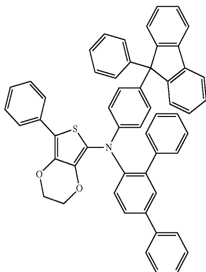
Compound 9
