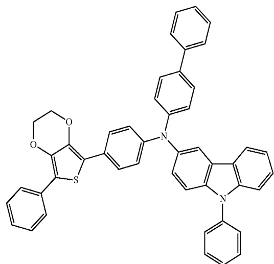
Compound 49
