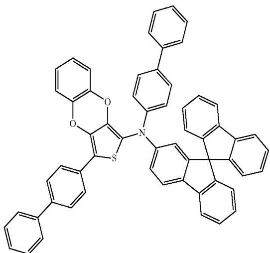
Compound 67
