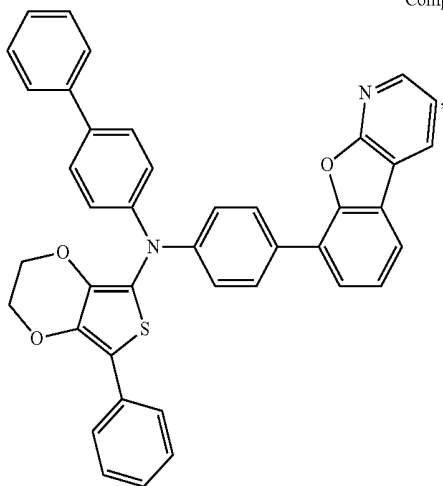
Compound 26
