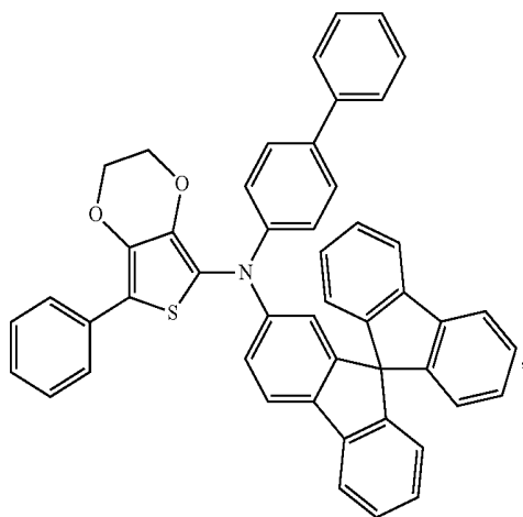
Compound 7
