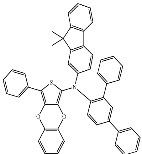
Compound 57
