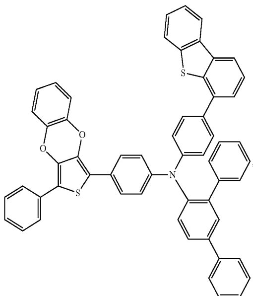
Compound 100
