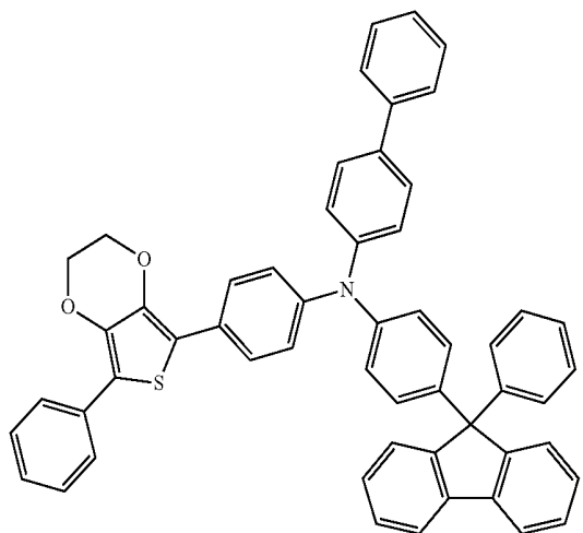
Compound 37
