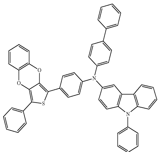
Compound 103
