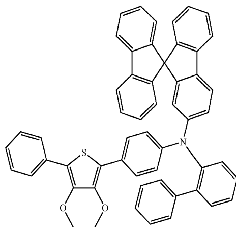
Compound 35
