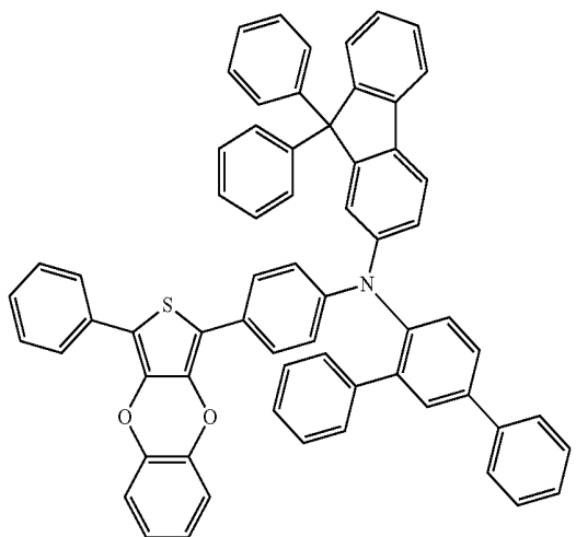
Compound 87
