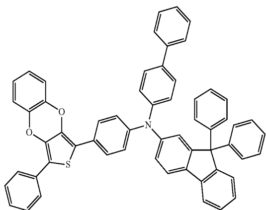
Compound 85
