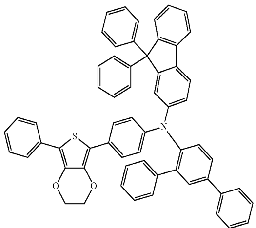
Compound 33
