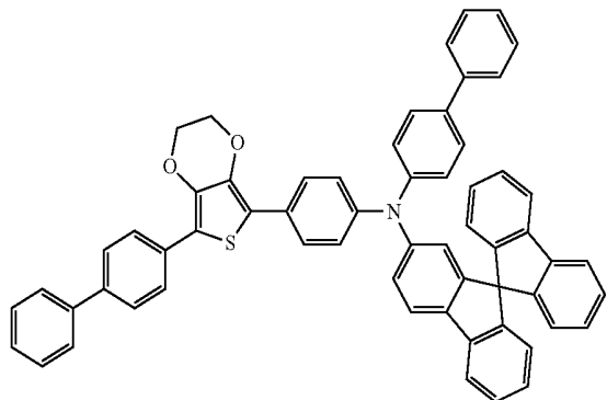
Compound 41
