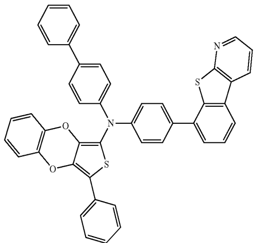
Compound 78
