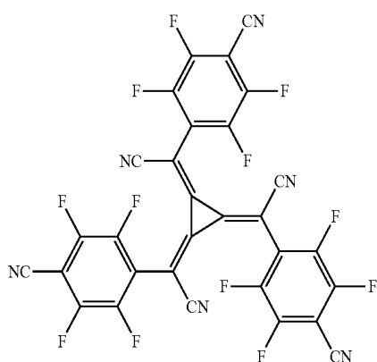
Compound X
