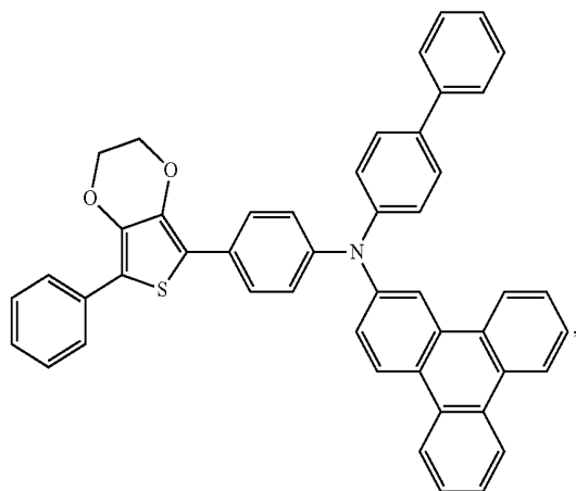
Compound 50
