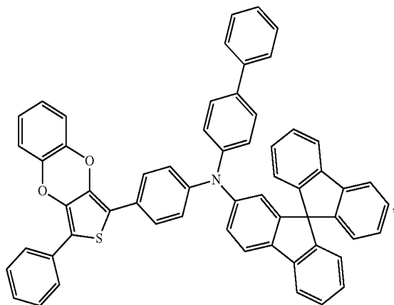
Compound 88
