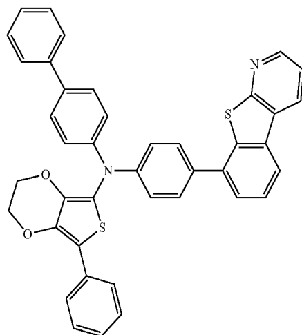
Compound 24
