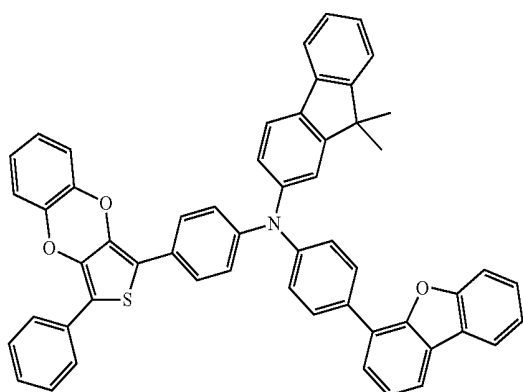
Compound 108
