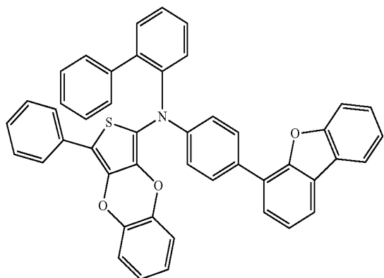
Compound 71
