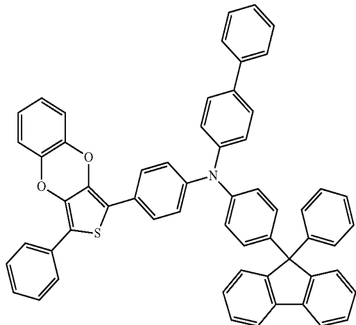
Compound 91
