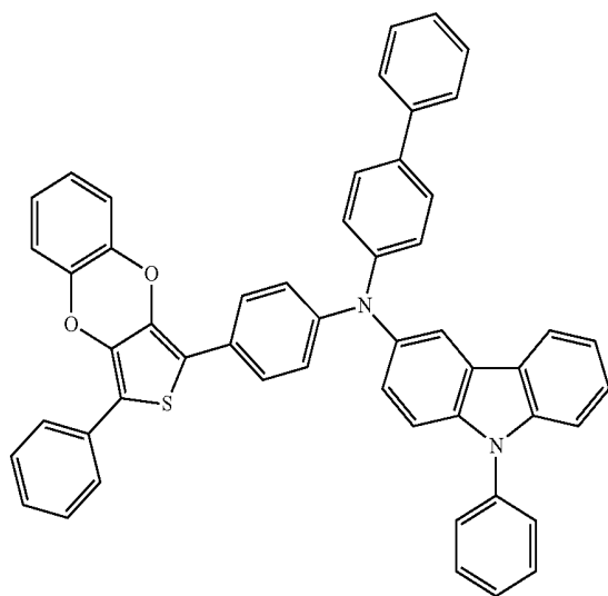
Compound 103
