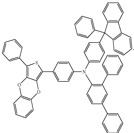
Compound 93
