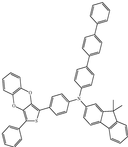
Compound 108
