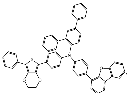
Compound 43
