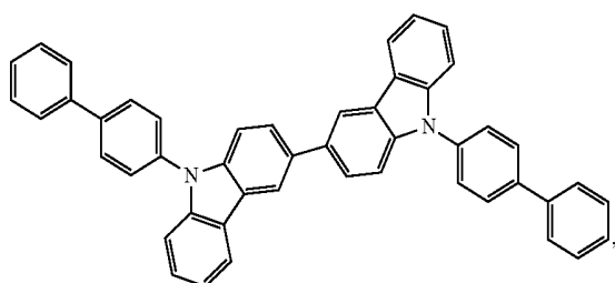
Compound H2
