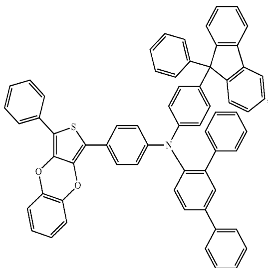
Compound 93
