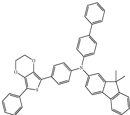
Compound 28
