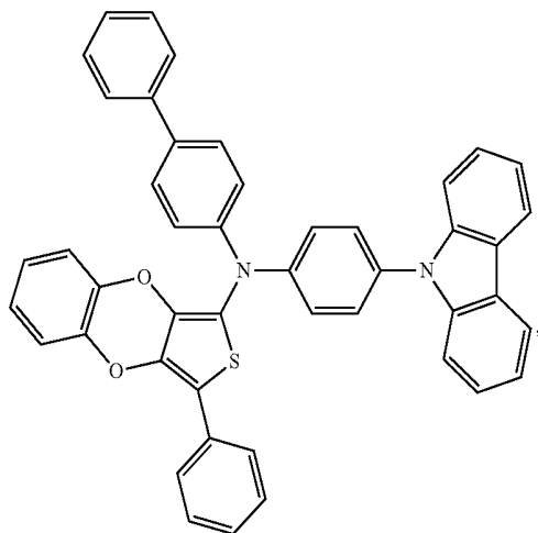
Compound 76
