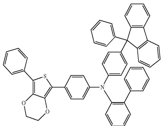
Compound 38
