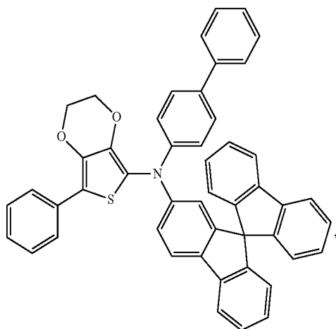
Compound 7
