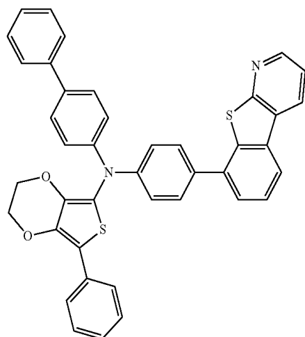
Compound 24
