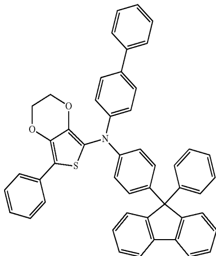
Compound 10
