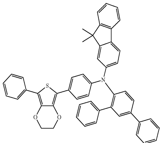
Compound 30
