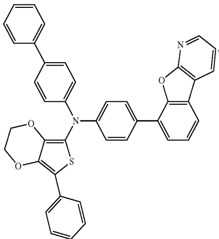
Compound 25
