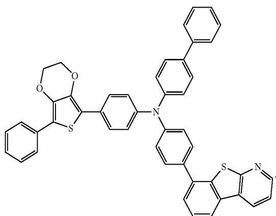
Compound 52
