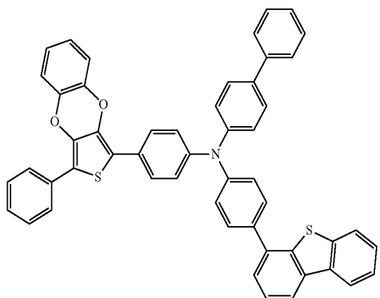
Compound 105
