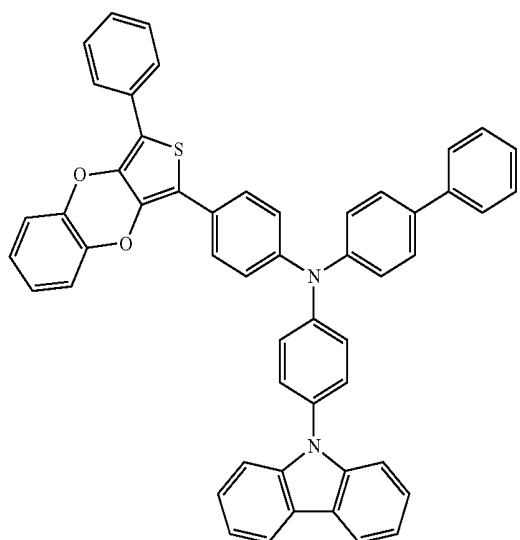
Compound 103
