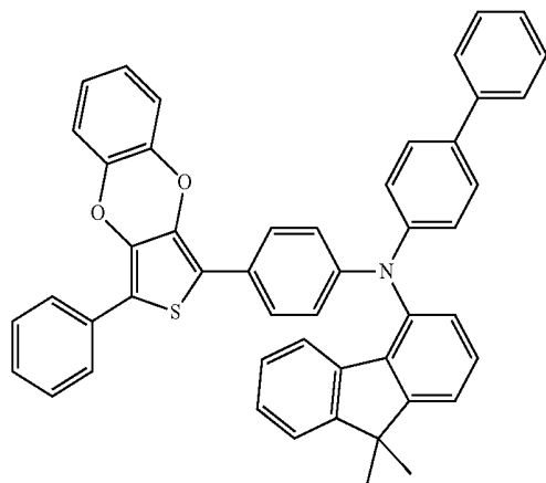
Compound 83
