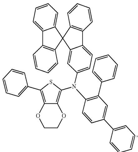
Compound 9
