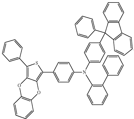
Compound 92
