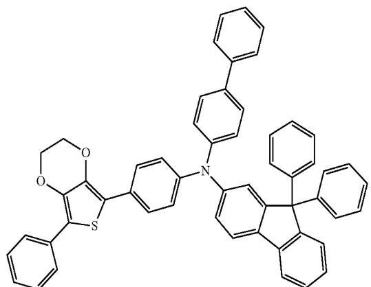
Compound 31
