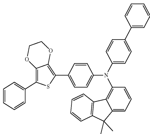
Compound 29
