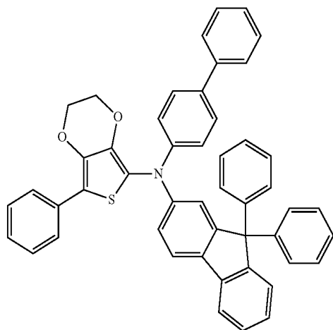
Compound 4
