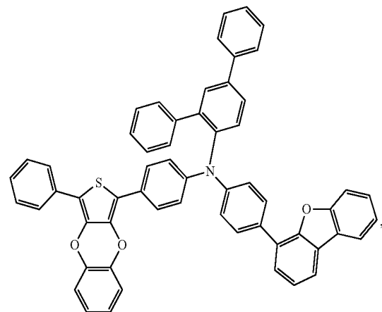
Compound 97
