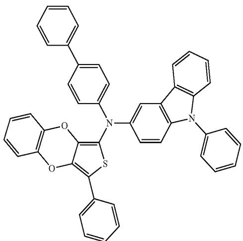
Compound 75
