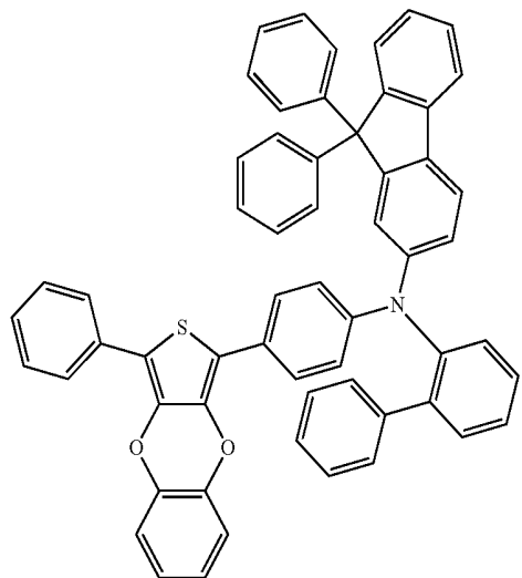
Compound 86
