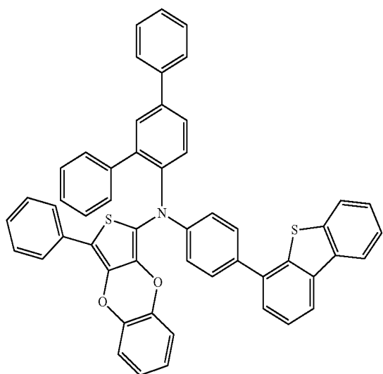
Compound 73
