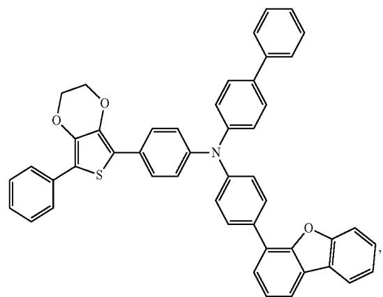
Compound 43
