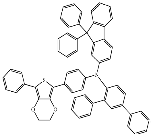
Compound 33
