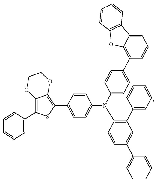
Compound 46
