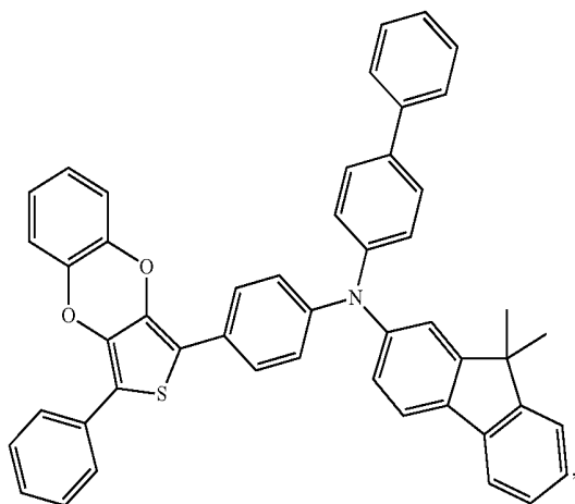
Compound 82
