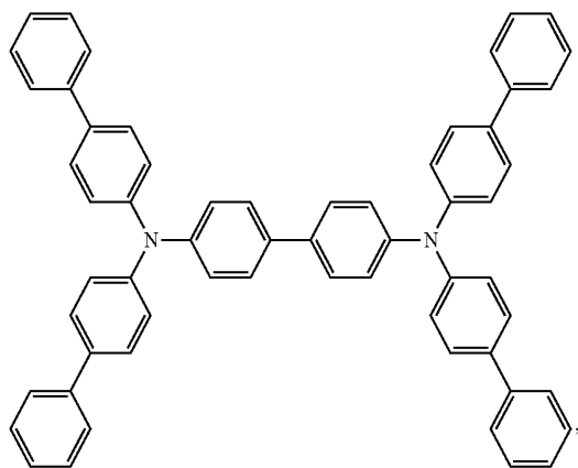
Compound 1
