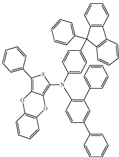
Compound 64
