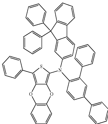
Compound 60
