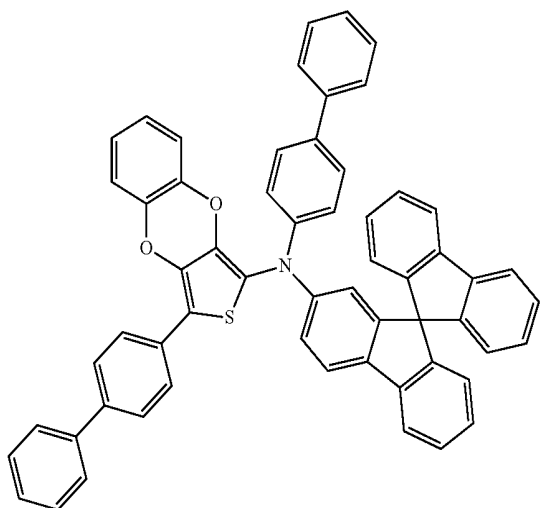
Compound 67
