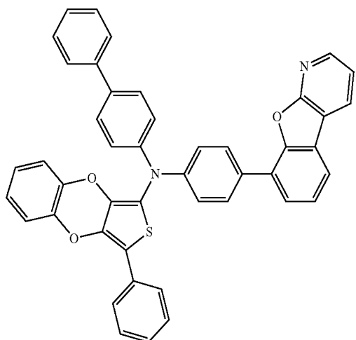
Compound 79
