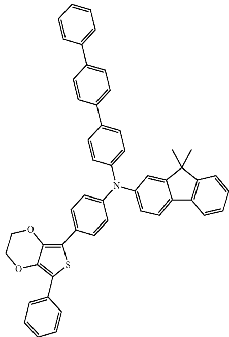
Compound 54
