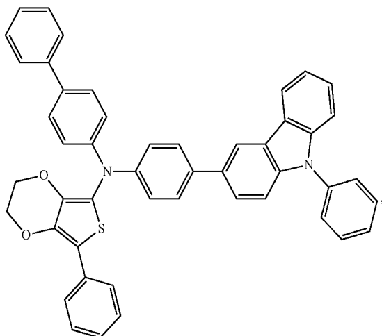
Compound 20
