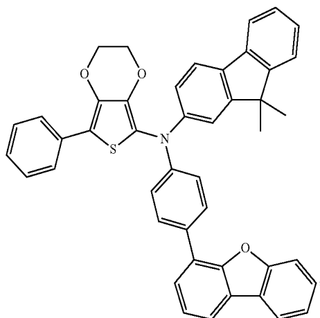
Compound 27
