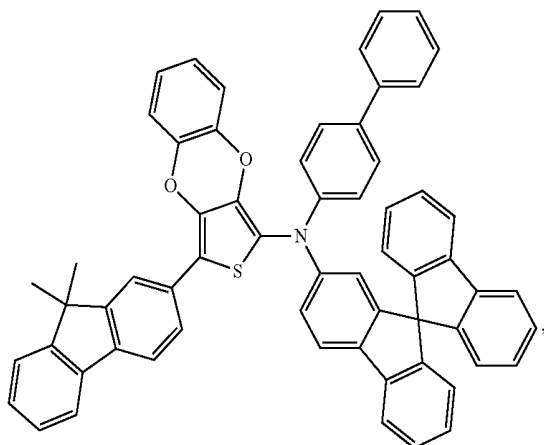
Compound 68
