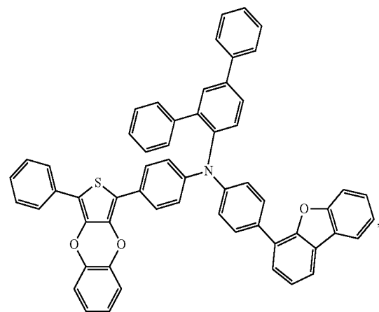
Compound 97
