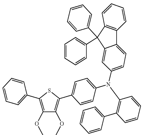
Compound 32
