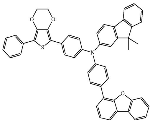
Compound 54
