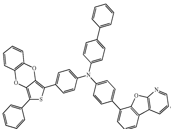
Compound 106
