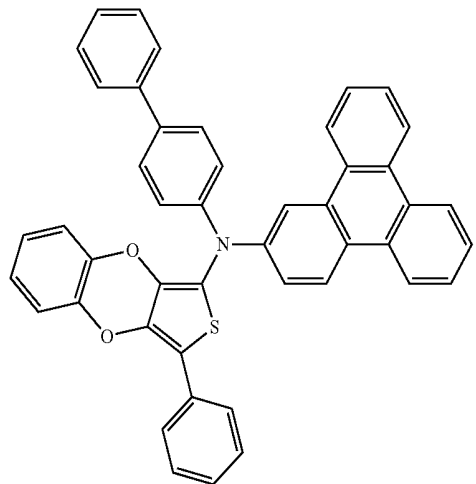
Compound 77
