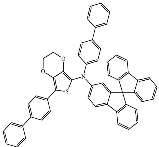
Compound 13
