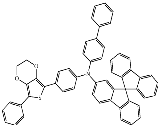
Compound 34
