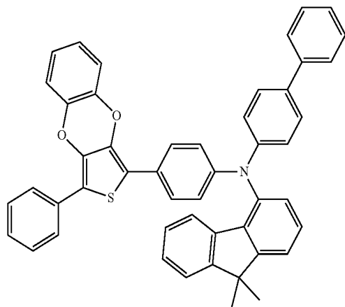
Compound 83
