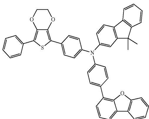
Compound 54
