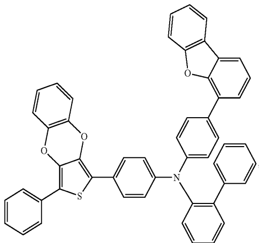
Compound 99
