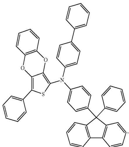
Compound 64
