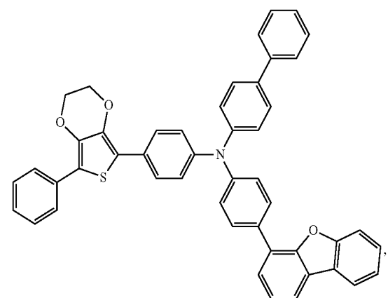
Compound 43
