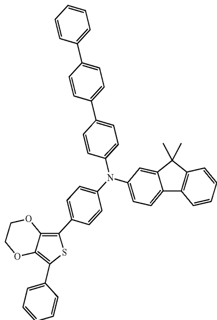
Compound 54
