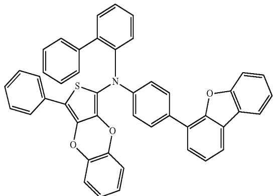
Compound 71
