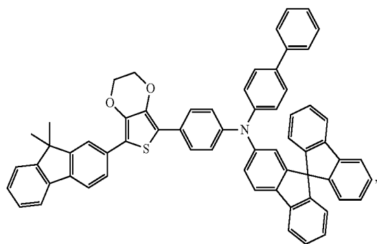
Compound 42
