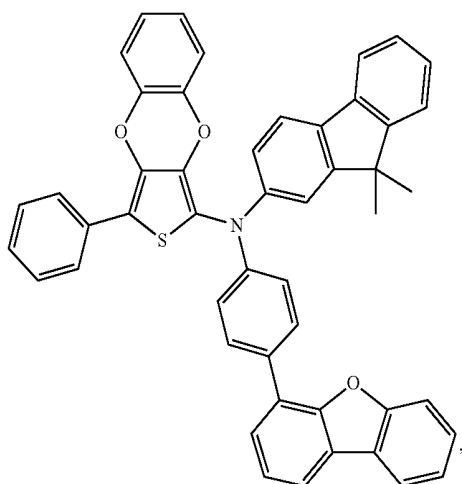
Compound 82
