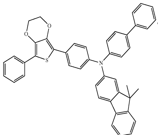
Compound 1
