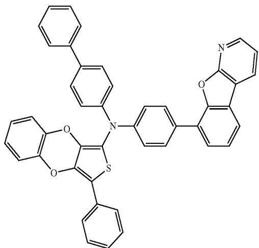
Compound 79
