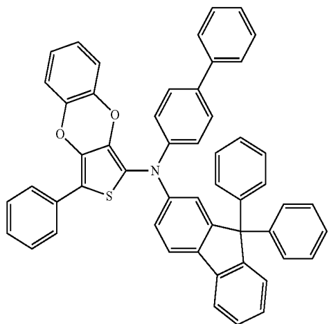
Compound 58
