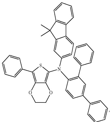
Compound 3
