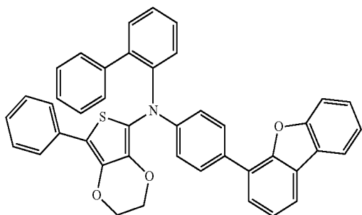
Compound 17
