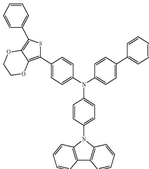
Compound 49
