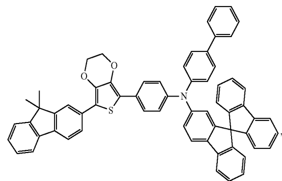
Compound 42
