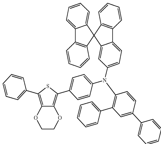
Compound 36
