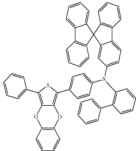
Compound 89
